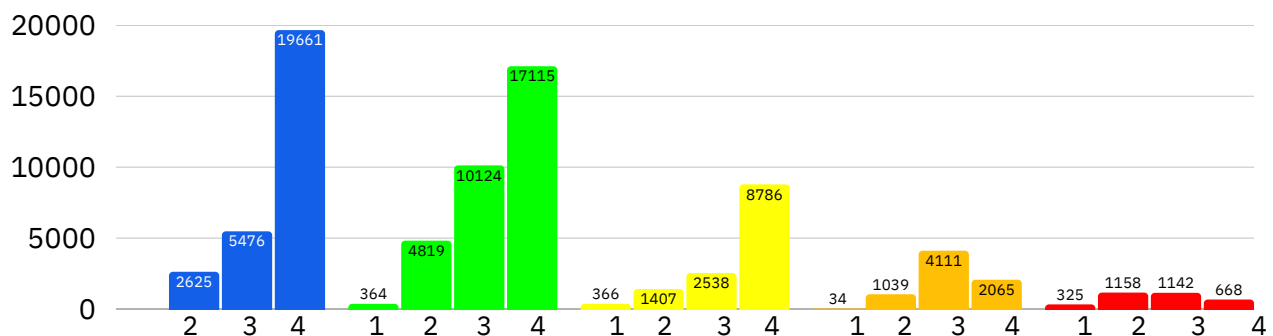
Figure 4: Distribution in rkm for the five HYMO classes within the size categories 1-4; 1=very large rivers, 2=large rivers, 3=medium-sized rivers, 4=small rivers (HYMO class 1 for the Danube (size category 1) cannot be found at all).
