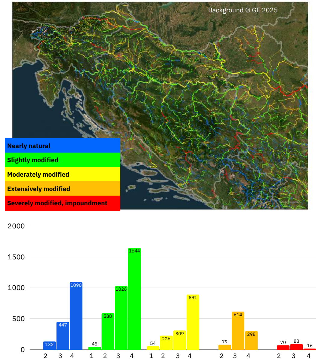
Figure 11: Distribution in rkm within the size categories 2-4; 2=large rivers, 3=medium-sized rivers, 4=small rivers (size category 1 for the Danube is not applicable).
