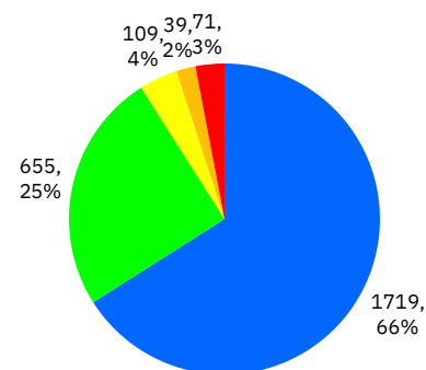
Figure 17: Montenegrin HYMO percentages and rkm distribution.
